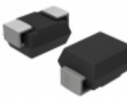
NP0640SBMCT3G ON Semiconductor THYRISTOR 58V 250A SMB
