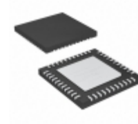
PIC24FJ64GA104T-I/ML Microchip Technology IC MCU 16BIT 64KB FLASH 44QFN
