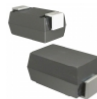
CDBA240L-HF Comchip Technology DIODE SCHOTTKY 40V 2A DO214AC
