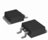
IRF3711SPBF Infineon Technologies MOSFET N-CH 20V 110A D2PAK
