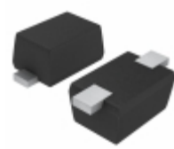
EDZTE618.2B LAPIS Semiconductor DIODE ZENER 8.2V 150MW EMD2
