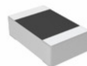
08051J1R3BBTTR AVX Corporation CAP THIN FILM 1.3PF 100V 0805
