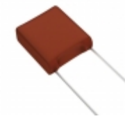
ECW-FA2J124J4 Panasonic Electronic Components CAP FILM 0.12UF 5% 630VDC RADIAL
