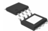
BD30HC5MEFJ-LBH2 LAPIS Semiconductor IC REG LINEAR 3V 1.5A 8HTSOP-J
