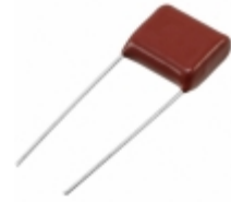
ECQ-E6184RKFB Panasonic Electronic Components CAP FILM 0.18UF 10% 630VDC RAD
