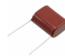
ECQ-E6185JFB Panasonic Electronic Components CAP FILM 1.8UF 5% 630VDC RADIAL
