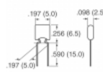
B37987F5104K068 EPCOS (TDK) CAP CER 0.1UF 50V X7R RADIAL
