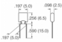
B37987F1473K054 EPCOS (TDK) CAP CER 0.047UF 100V X7R RADIAL
