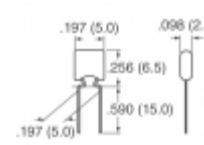
B37987F5104K031 EPCOS (TDK) CAP CER 0.1UF 50V X7R RADIAL
