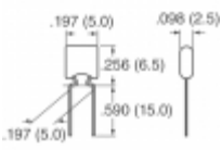
B37987F5104K058 EPCOS (TDK) CAP CER 0.1UF 50V X7R RADIAL
