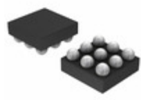
NCP4894FCT1 ON Semiconductor IC AMP AUDIO PWR 1W DIFF 9FLPCHP
