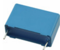
B32523Q3684J EPCOS (TDK) CAP FILM 0.68UF 5% 250VDC RADIAL
