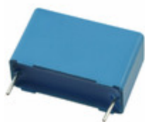
B32523Q475K EPCOS (TDK) CAP FILM 4.7UF 10% 63VDC RADIAL
