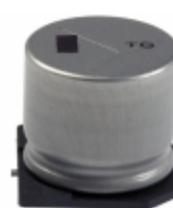
EEV-TG1E222M Panasonic Electronic Components CAP ALUM 2200UF 20% 25V SMD
