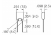
B37985N5155M000 EPCOS (TDK) CAP CER 1.5UF 50V Z5U RADIAL
