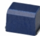
NLC453232T-1R0K-PF TDK Corporation FIXED IND 1UH 1.05A 110 MOHM SMD
