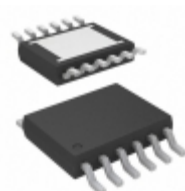
LT3065EMSE#TRPBF ADI (Analog Devices, Inc.) IC REG LIN POS ADJ 500MA 12MSOP
