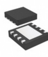
24LC02BT-I/MC Microchip Technology IC EEPROM 2KBIT 400KHZ 8DFN
