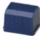
NLC453232T-331K-PF TDK Corporation FIXED IND 330UH 90MA 13 OHM SMD
