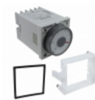
PM4HA-H-24VSW Panasonic RELAY TIME DELAY 500HR 5A 250V
