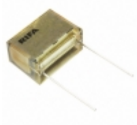
PME271YE6150KR30 KEMET CAP FILM 0.15UF 10% 1KVDC RADIAL
