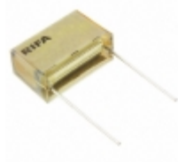
PME271YD6100MR30 KEMET CAP FILM 0.1UF 20% 1KVDC RADIAL
