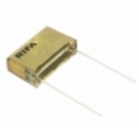
PME271YD5470MR30 KEMET CAP FILM 0.047UF 20% 1KVDC RAD
