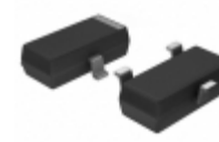
MA3ZD1200L Panasonic Electronic Components DIODE SCHOTTKY 20V 700MA SMINI3
