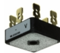
VS-26MT40 Electro-Films (EFI) / Vishay RECTIFIER BRIDGE 400V 25A D-63
