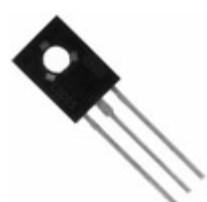
MJE350 STMicroelectronics TRANS PNP 300V 0.5A SOT-32
