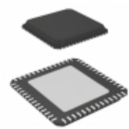
LAN9303-ABZJ Microchip Technology IC ETHER SW 3PORT 16BIT 56QFN
