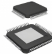
LAN9252TI/PT Microchip Technology IC ETHERCAT CTRLR 10/100 64TQFP
