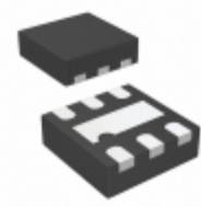
MIC5371-SGYMT-TR Microchip Technology IC REG LDO 3.3V/2.8V 0.15A 6TMLF
