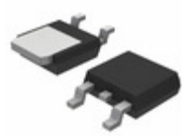
NJVMJD128T4G ON Semiconductor TRANS PNP DARL 120V 8A DPAK-4
