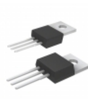
IXFP5N100PM IXYS MOSFET N-CH 1000V 2.3A TO-220
