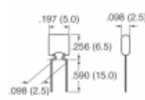
B37987M5104K058 EPCOS (TDK) CAP CER 0.1UF 50V X7R RADIAL
