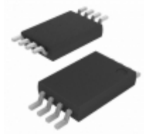
IRF7702GTRPBF Infineon Technologies MOSFET P-CH 12V 8A 8-TSSOP
