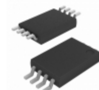
AT24C01C-XHM-B Microchip Technology IC EEPROM 1KBIT 1MHZ 8TSSOP
