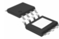
BD15HA3WEFJ-E2 Rohm Semiconductor IC REG LDO 1.5V 0.3A 8-HTSOP
