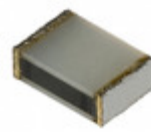
ECW-U2683V16 Panasonic Electronic Components CAP FILM 0.068UF 5% 250VDC 2416
