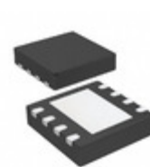
MCP4141-502E/MF Microchip Technology IC POT DGTL SNGL 5K SPI 8DFN
