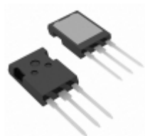
IXGX35N120B IXYS IGBT 1200V 70A 350W PLUS247
