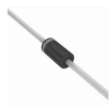
1N4750A-TR Vishay Semiconductor Diodes Division DIODE ZENER 27V 1.3W DO41
