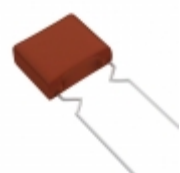
ECW-F2104RJA Panasonic Electronic Components CAP FILM 0.1UF 5% 250VDC RADIAL
