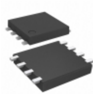
ECH8656-TL-H ON Semiconductor MOSFET N-CH 20V 7.5A ECH8
