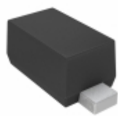
VDZT2R16B Rohm Semiconductor DIODE ZENER 16V 100MW VMD2
