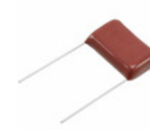
ECQ-E6474KFB Panasonic Electronic Components CAP FILM 0.47UF 10% 630VDC RAD
