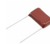
ECQ-E6474KF Panasonic Electronic Components CAP FILM 0.47UF 10% 630VDC RAD
