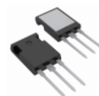
IXFR150N15 IXYS MOSFET N-CH 150V 105A ISOPLUS247
