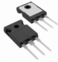
FGH40T65SHDF_F155 Fairchild/ON Semiconductor IGBT 650V 80A 268W TO-247-3
