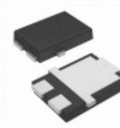
VS-10CSH02-M3/87A Electro-Films (EFI) / Vishay DIODE ARRAY GP 200V 5A TO277A
