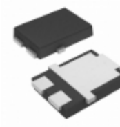
VS-10CSH02-M3/86A Vishay Semiconductor Diodes Division DIODE ARRAY GP 200V 5A TO277A
