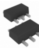
MCP1804T-2502I/MT Microchip Technology IC REG LDO 2.5V 0.1A SOT89-5
