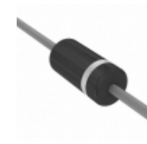
P6KE400A-E3/73 Vishay Semiconductor Diodes Division TVS DIODE 342VWM 548VC DO204AC
