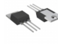
L6006L656 Littelfuse Inc. TRIAC SENS GATE 600V 6A TO220
