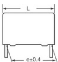
B32922C3223K000 EPCOS CAP FILM 0.022UF 10% 305VAC RAD
