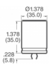
MAL215953681E3 Vishay BC Components CAP ALUM 680UF 20% 250V SNAP
