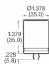
MAL215953821E3 Vishay BC Components CAP ALUM 820UF 20% 250V SNAP
