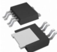
BA33C18FP-E2 LAPIS Semiconductor IC REG LDO 3.3V/1.8V 1A TO252-5
