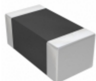
AMCV-1206H-380-T Abracon LLC VARISTOR 50V 250A 1206
