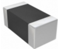
AMCV-1206H-300-T Abracon LLC VARISTOR 42V 250A 1206
