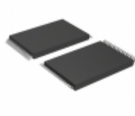
AT49F001T-70VC Microchip Technology IC FLASH 1MBIT 70NS 32VSOP
